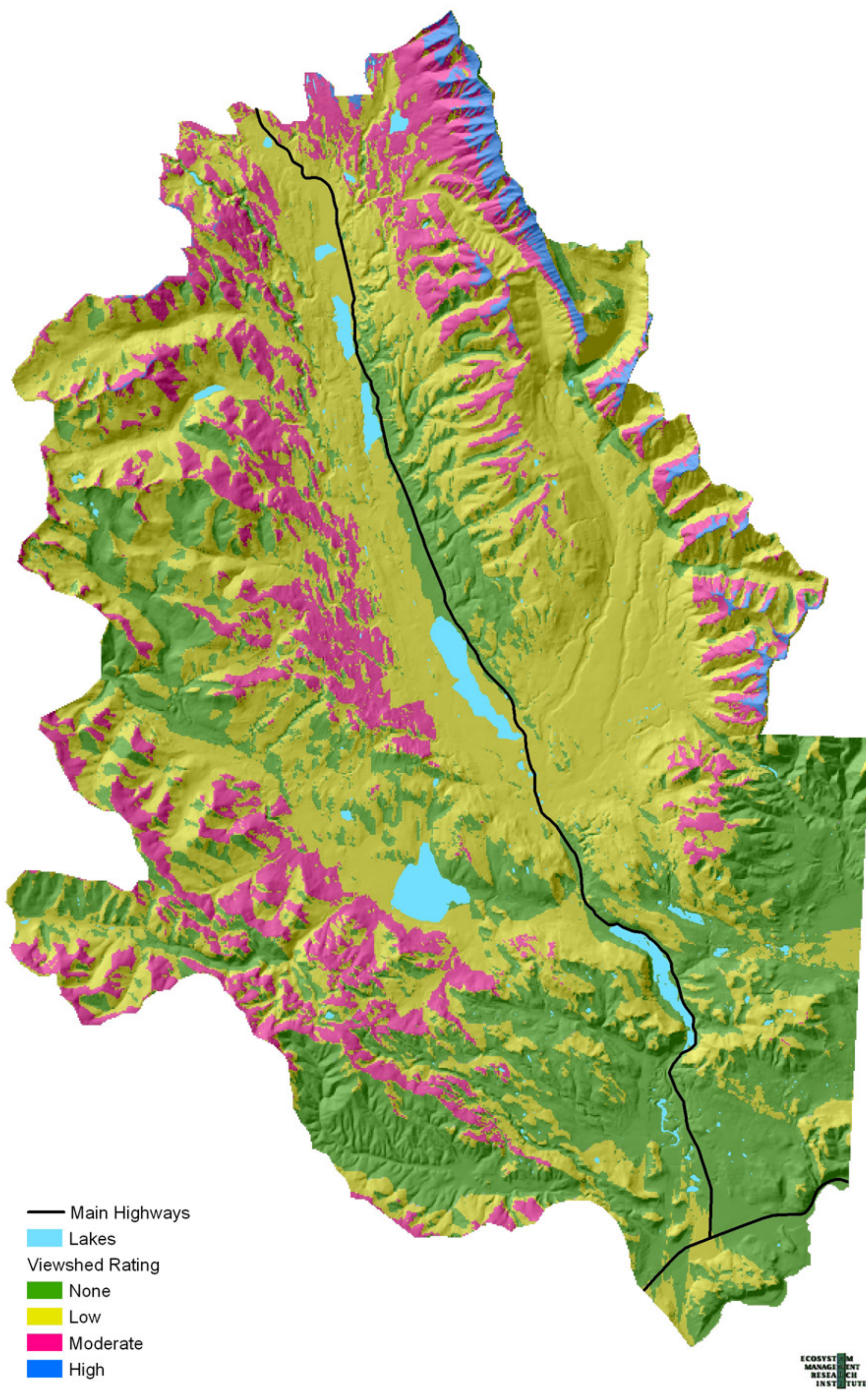
Figure 30. Viewshed of Peaks in the Clearwater Watershed (Derived from USGS NED, 2005).
