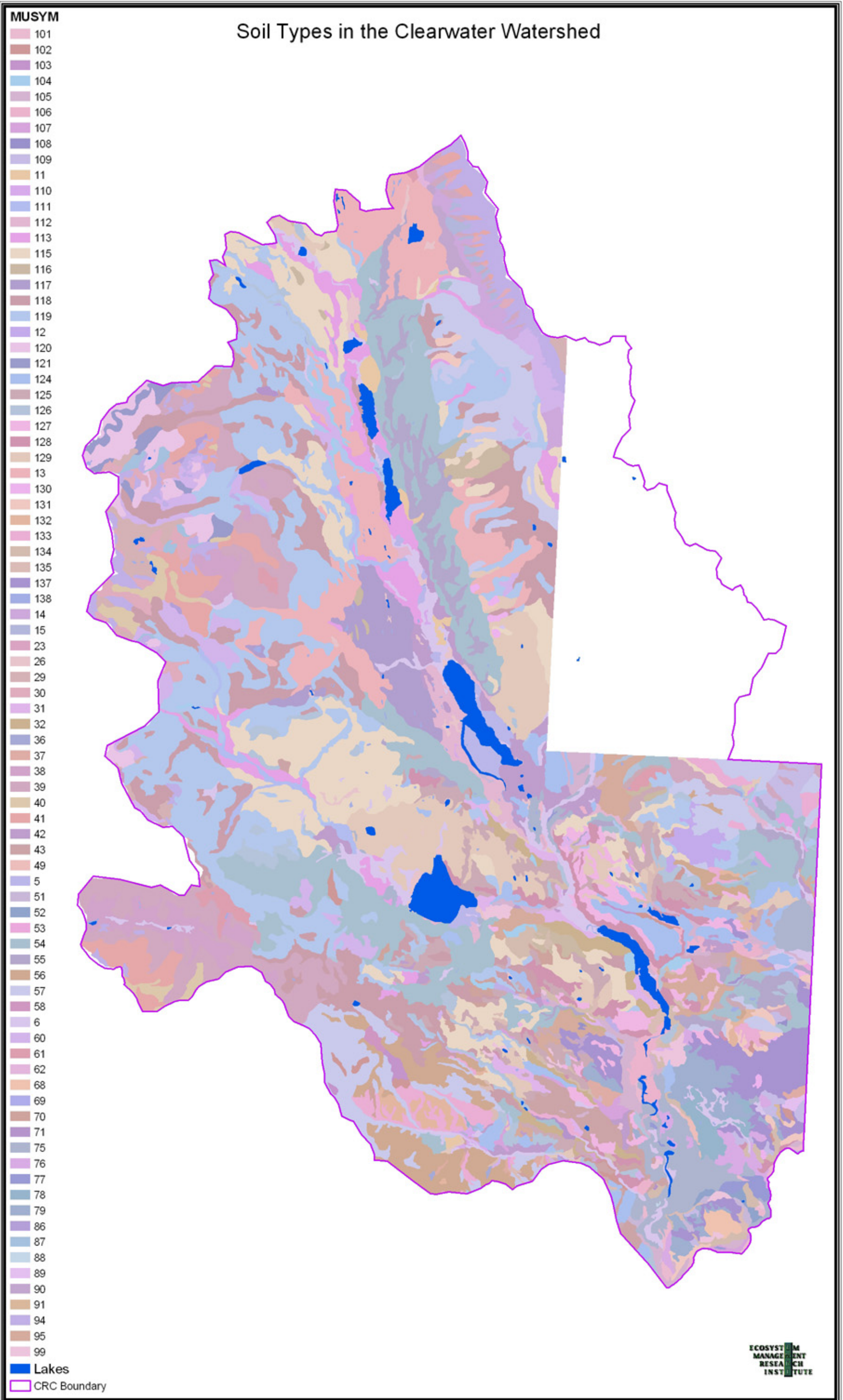
Figure 3. Soils Types in the Clearwater Watershed (USDANRCS, SSURGO, 2006).
