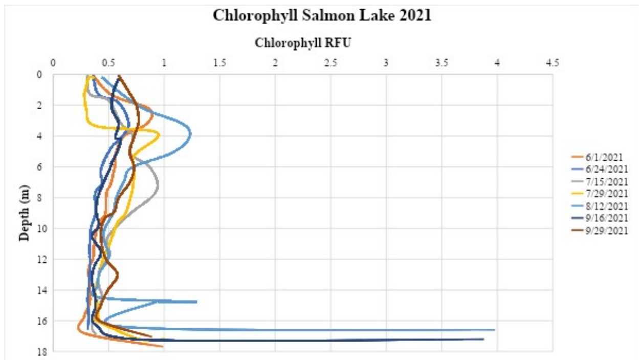
Figure 23. Chlorophyll (RFU) profile recorded at one site in Salmon Lake, from June through September 2021.
