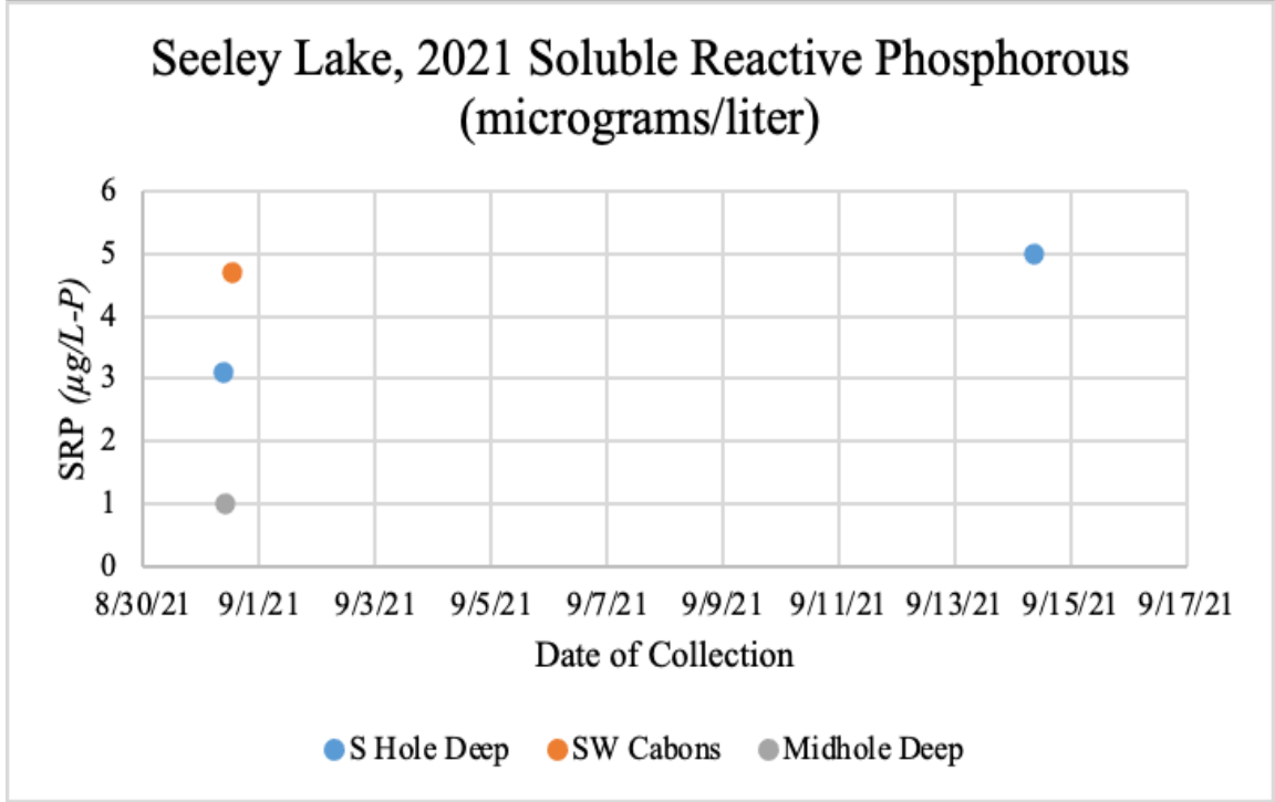
Figure 38. Soluble Reactive Phosphorus in Seeley Lake in 2021.
