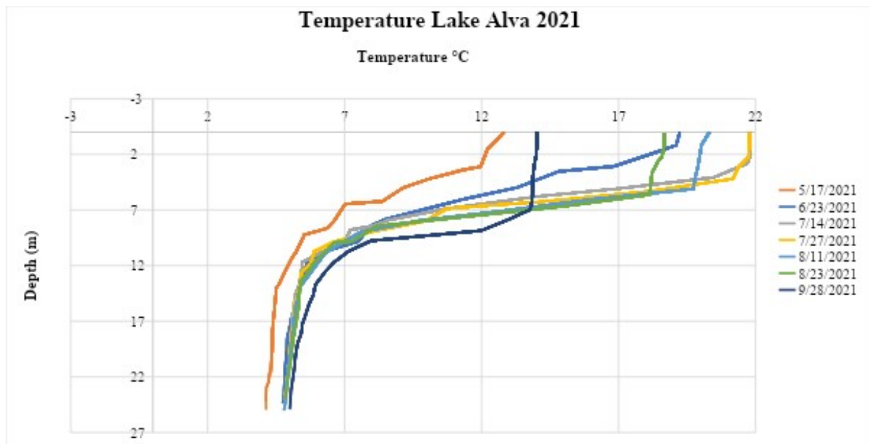
Figure 3. Temperature (°C) profile recorded at one site in Lake Alva, from May through September 2021.
