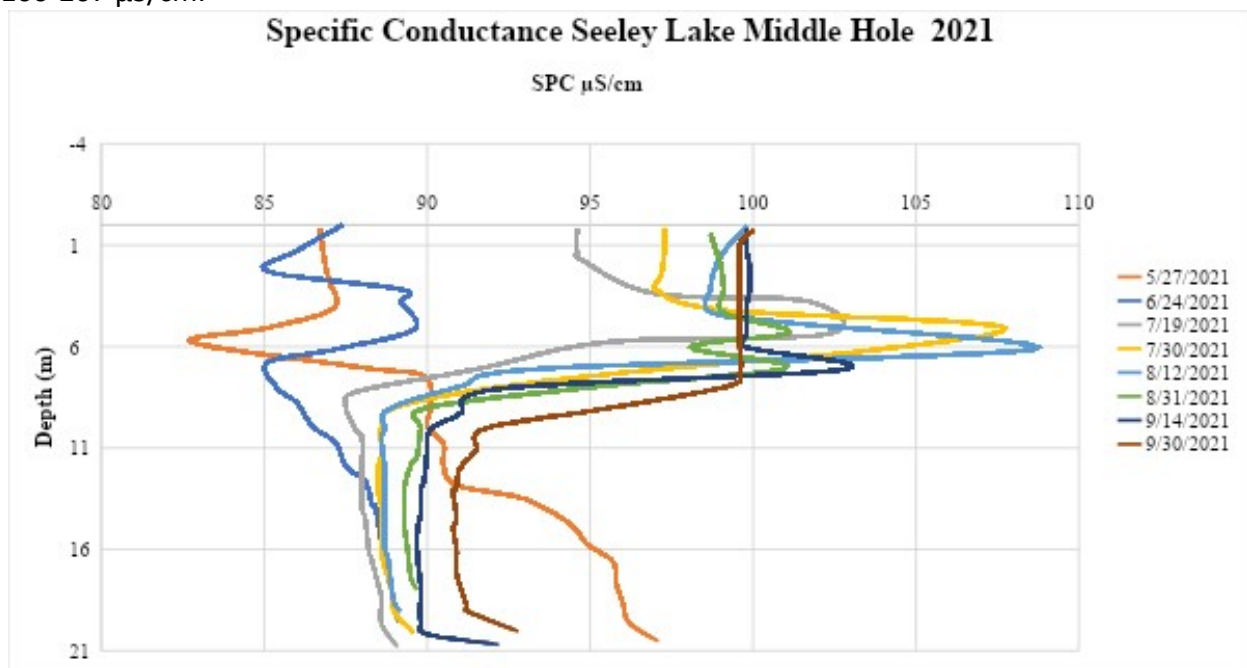
Figure 31a. Conductivity ( \mu\text{S}/\text{cm} ) profile recorded on the Middle Hole of Seeley Lake , from May through September 2021.
